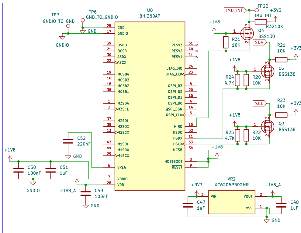
BHI260 Inertial Measurement Unit Circuit
