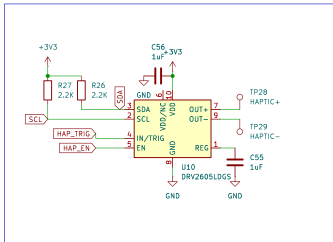
DRV2605 Haptic Driver Circuit
