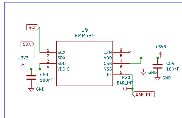
BMP585 Barometric Pressure Sensor Circuit
